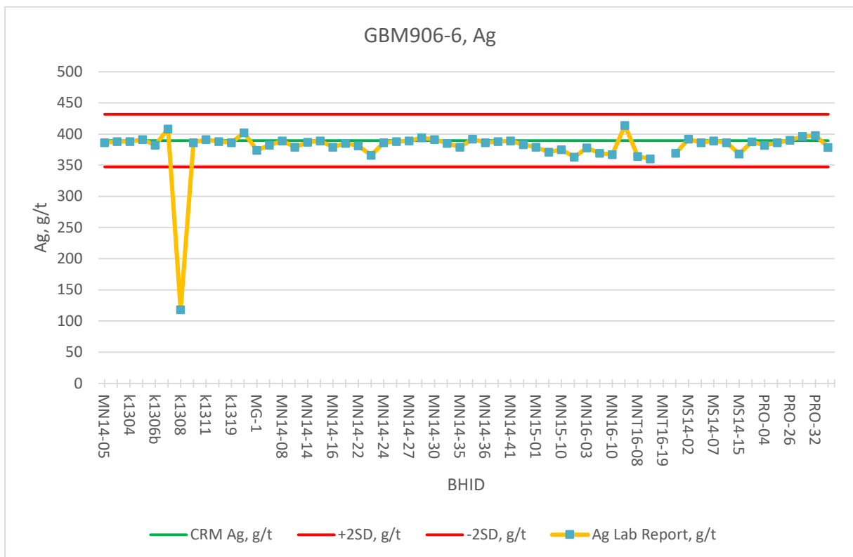
Figure 11.48: GBM 906-6, Ag, CRM Assaying Results
