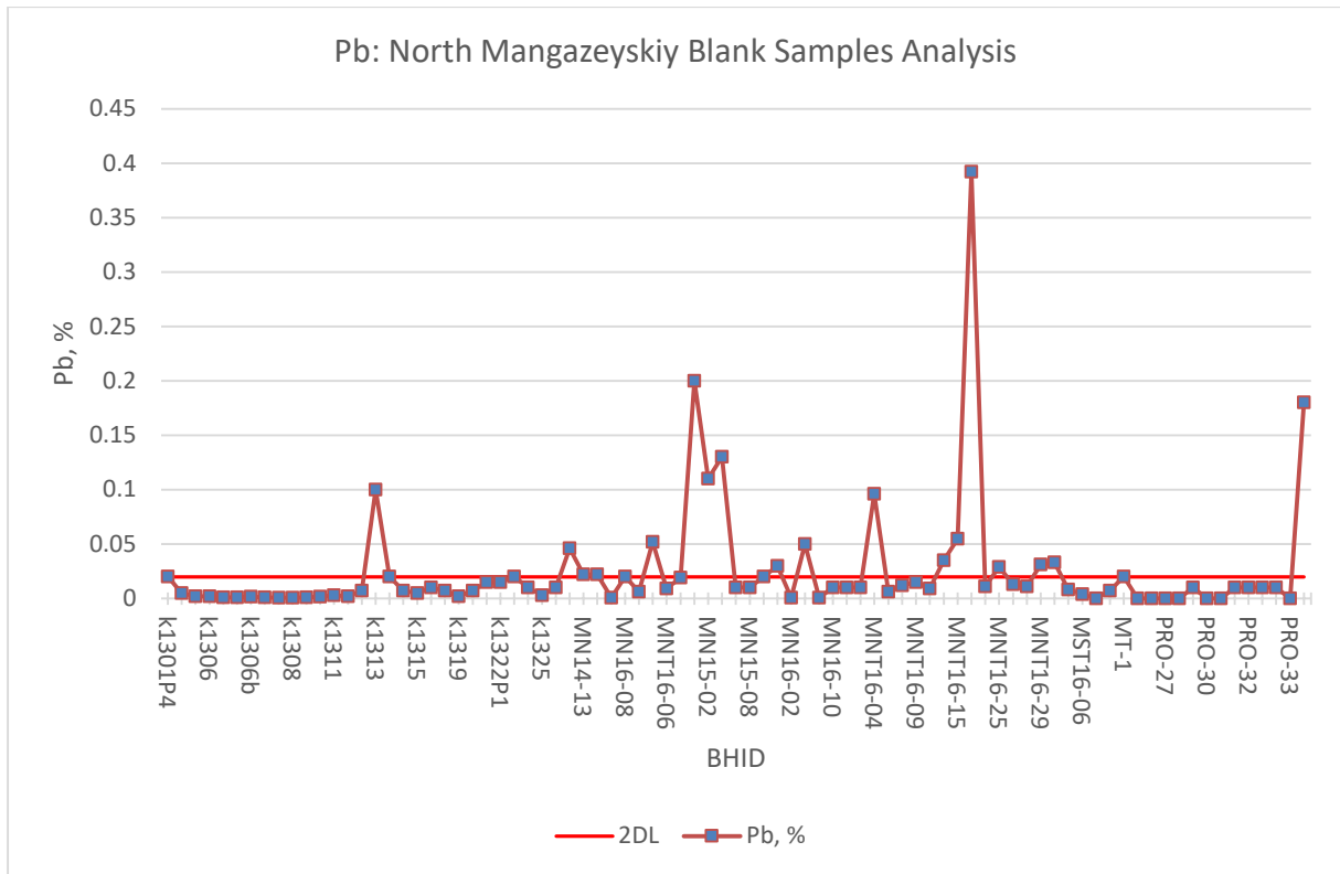
Figure 11.43: Blank Samples Analysed for Pb on North Mangazeyskiy
