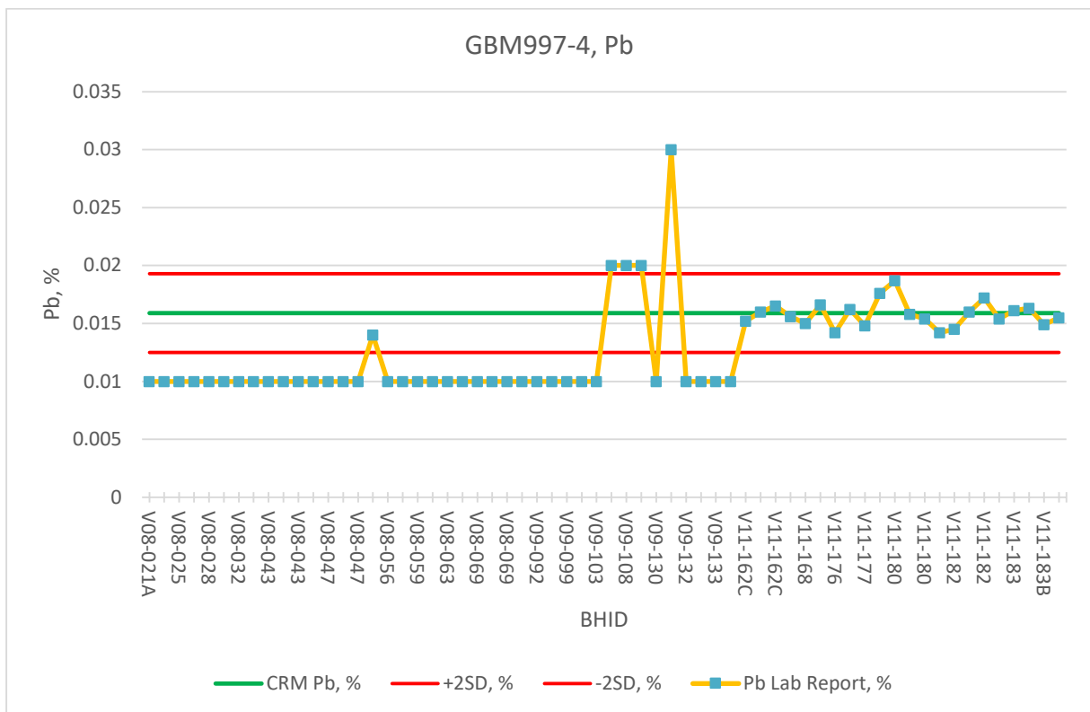
Figure 11.23: GBM 997-4, Pb, CRM Assaying Results
