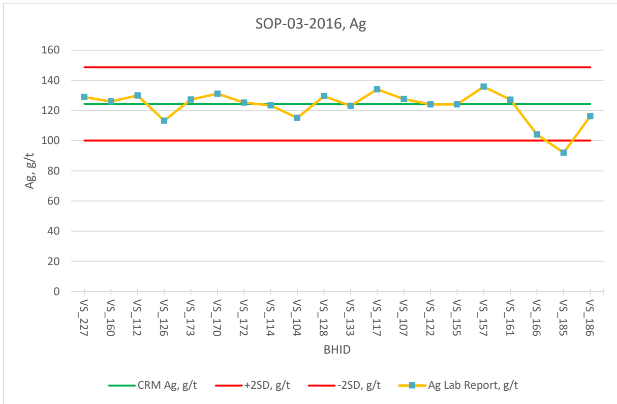
Figure 11.32: SOP-03-2016, Ag, CRM Assaying Results
