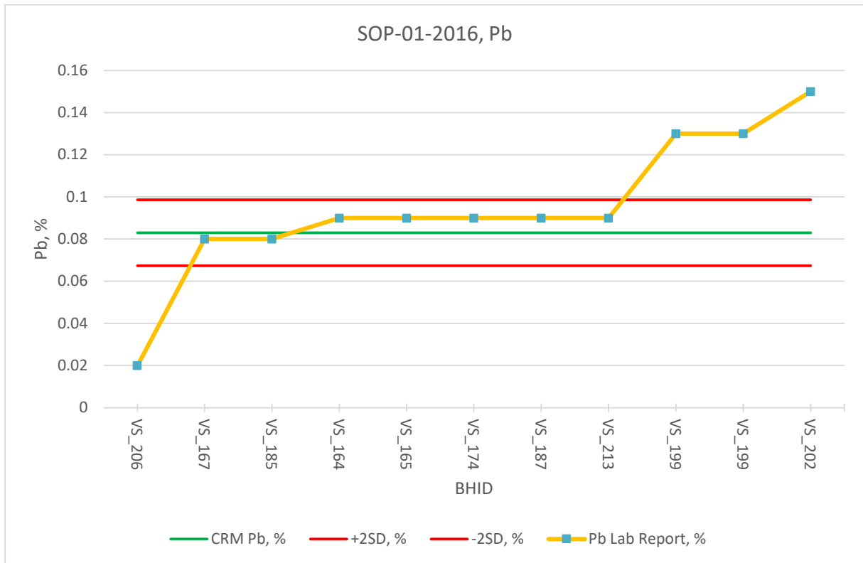
Figure 11.27: SOP-01-2016, Pb, CRM Assaying Results
