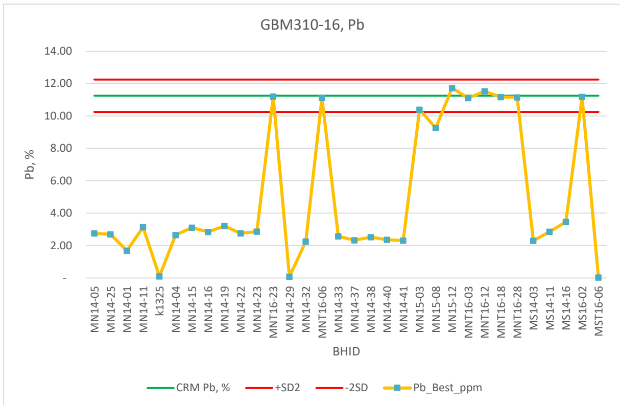
Figure 11.46: GBM 310-16, Pb, CRM Assaying Results
