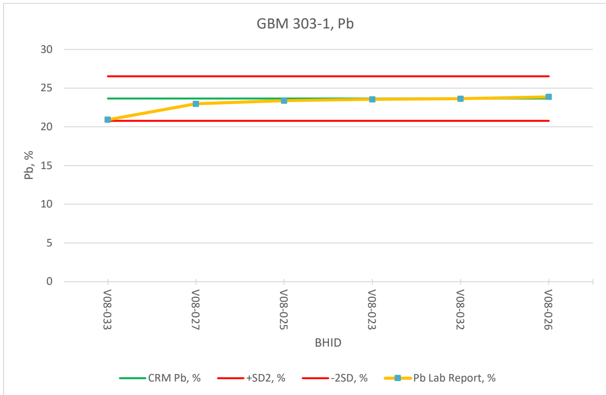
Figure 11.7: GBM 303-1, Pb, CRM Assaying Results
