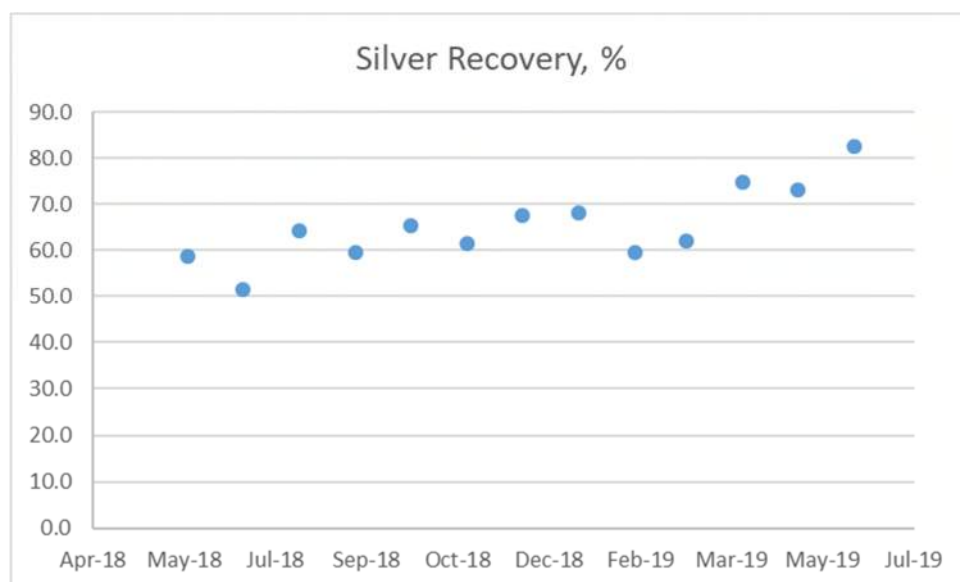
Figure 17.3: Final Silver Recovery
