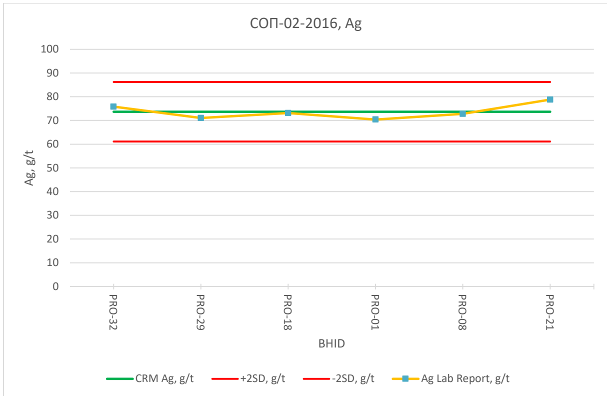
Figure 11.59: SOP-02-2016, Ag, CRM Assaying Results
