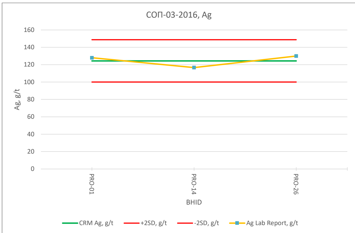
Figure 11.62: SOP-03-2016, Ag, CRM Assaying Results
