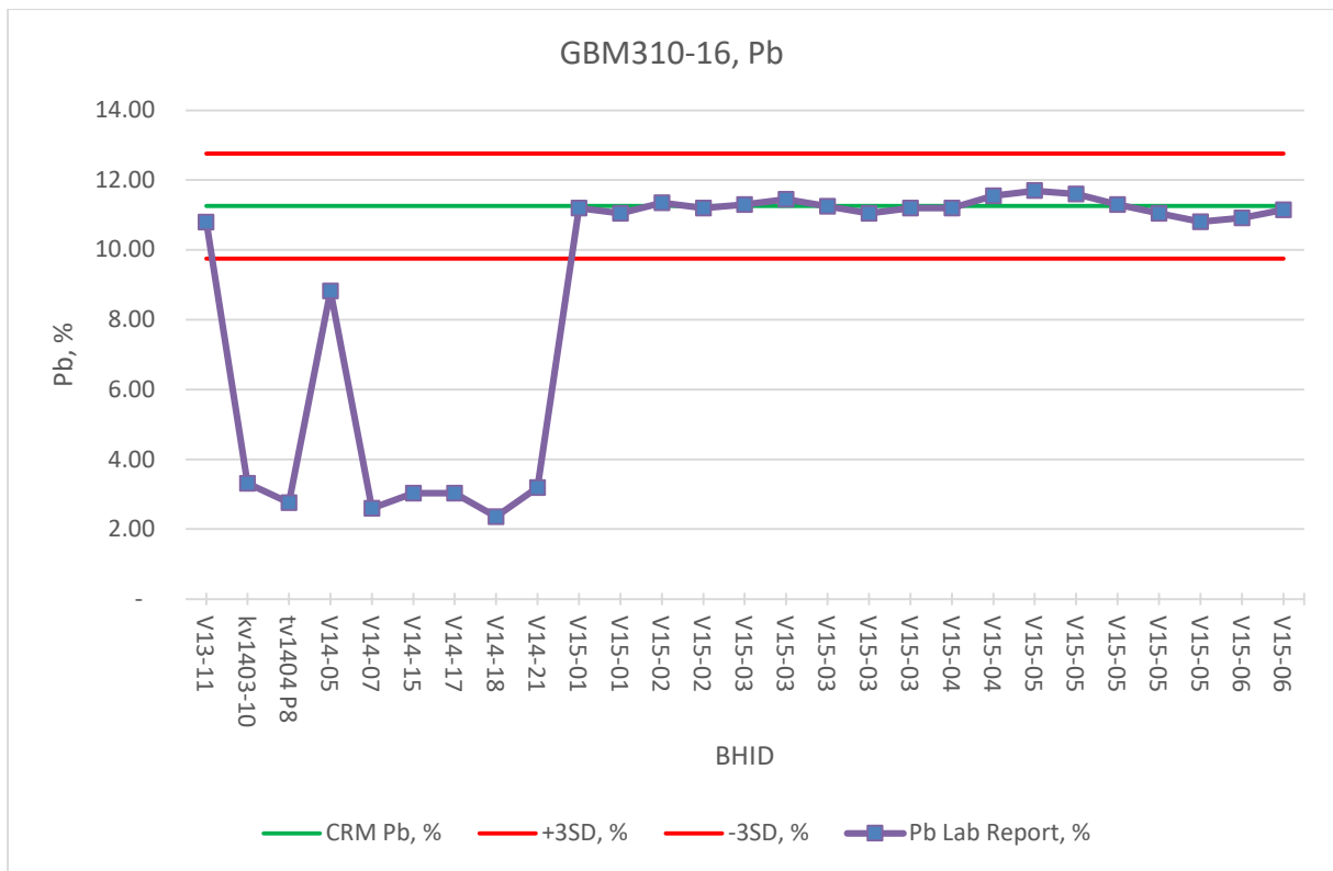
Figure 11.10: GBM 310-16, Pb, CRM Assaying Results
