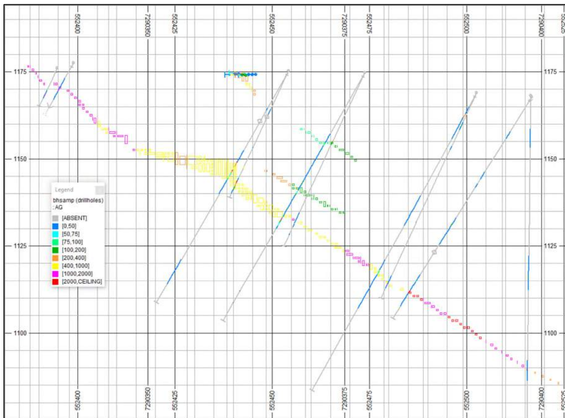
Figure 14.35: Block Model Grades vs Original Samples
