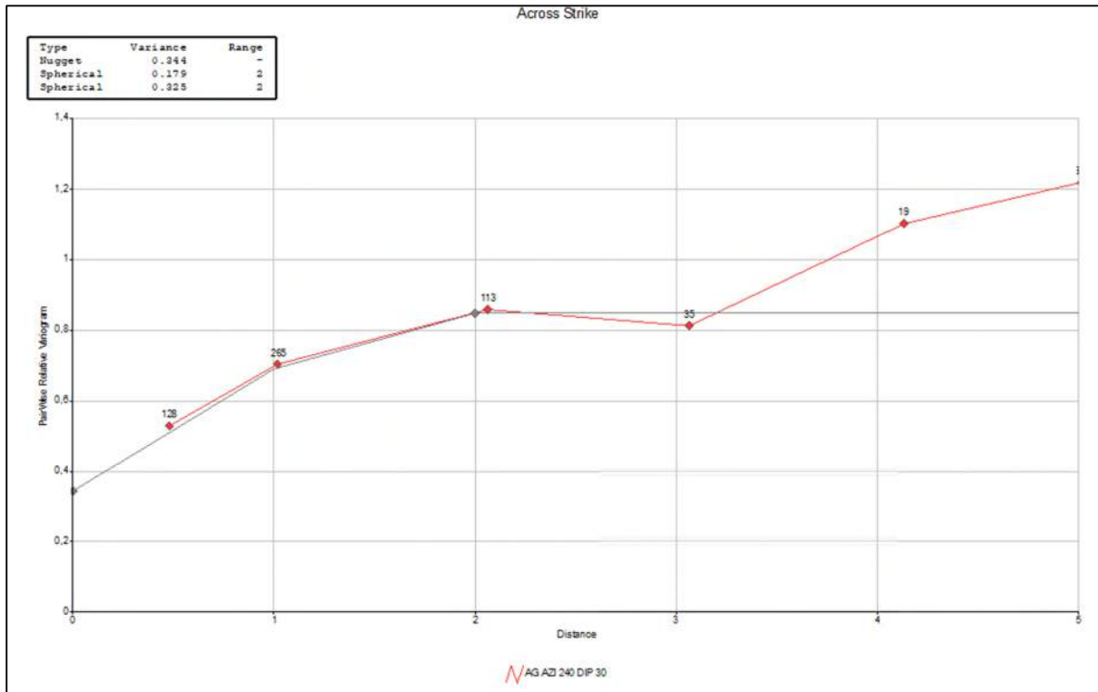
Figure 14.32: Ag Modelled Variogram, Zone 1, Across the Strike
