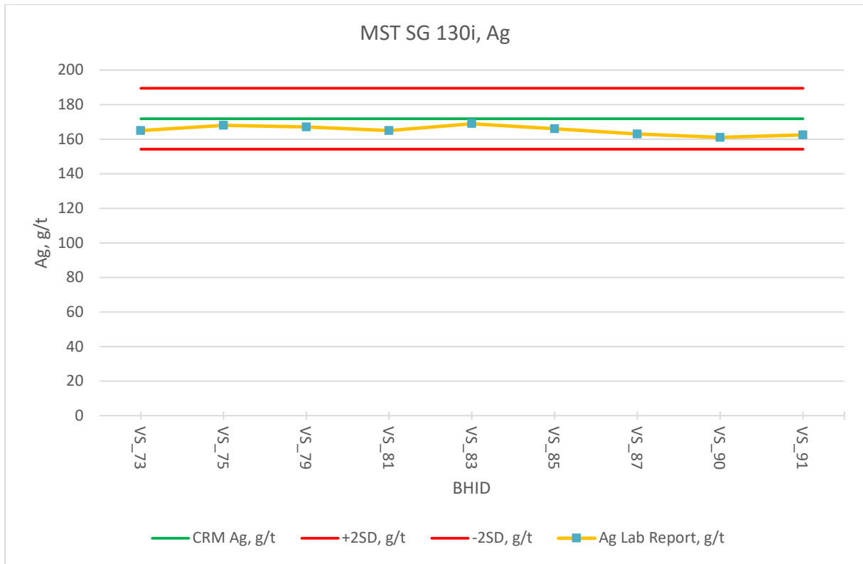
Figure 11.34: MST SG 130i, Ag, CRM Assaying Results
