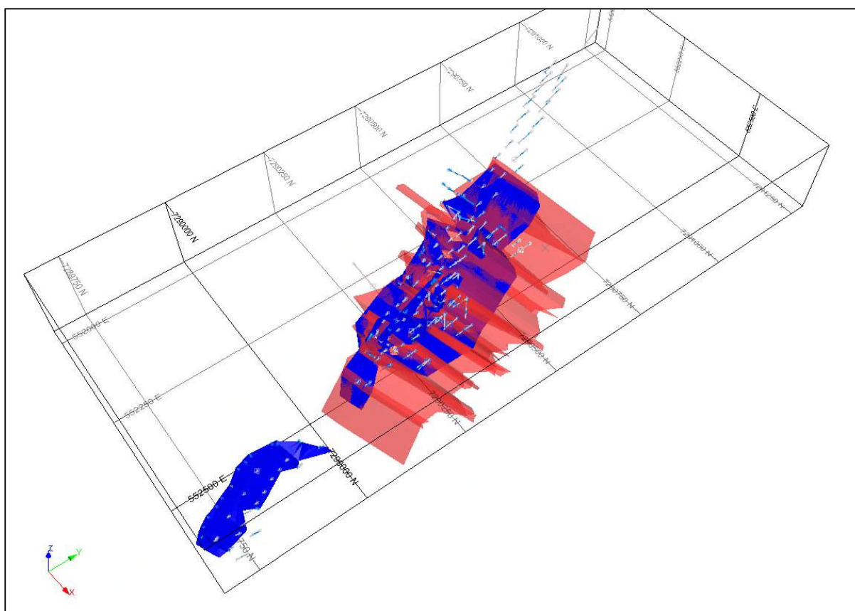
Figure 14.38: Wireframe Models of TT (red) and WAI (blue) with workings at Mangazeisky North
