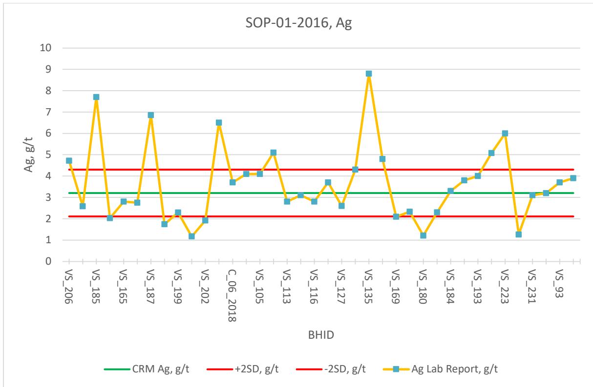
Figure 11.26: SOP-01-2016, Ag, CRM Assaying Results
