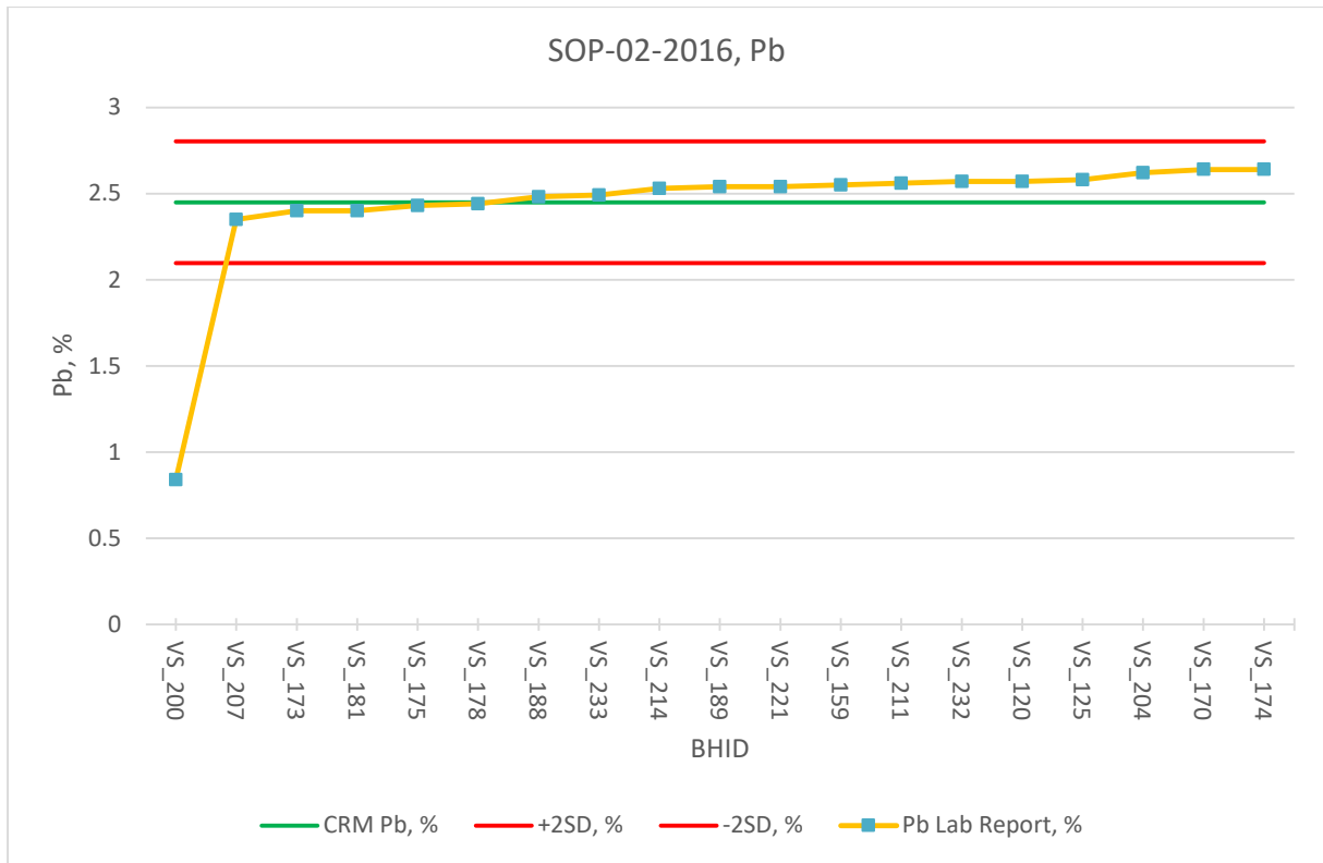
Figure 11.30: SOP-02-2016, Pb, CRM Assaying Results
