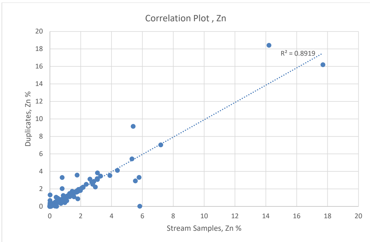
Figure 11.41: Correlation Plot for Field Duplicates, Zn
