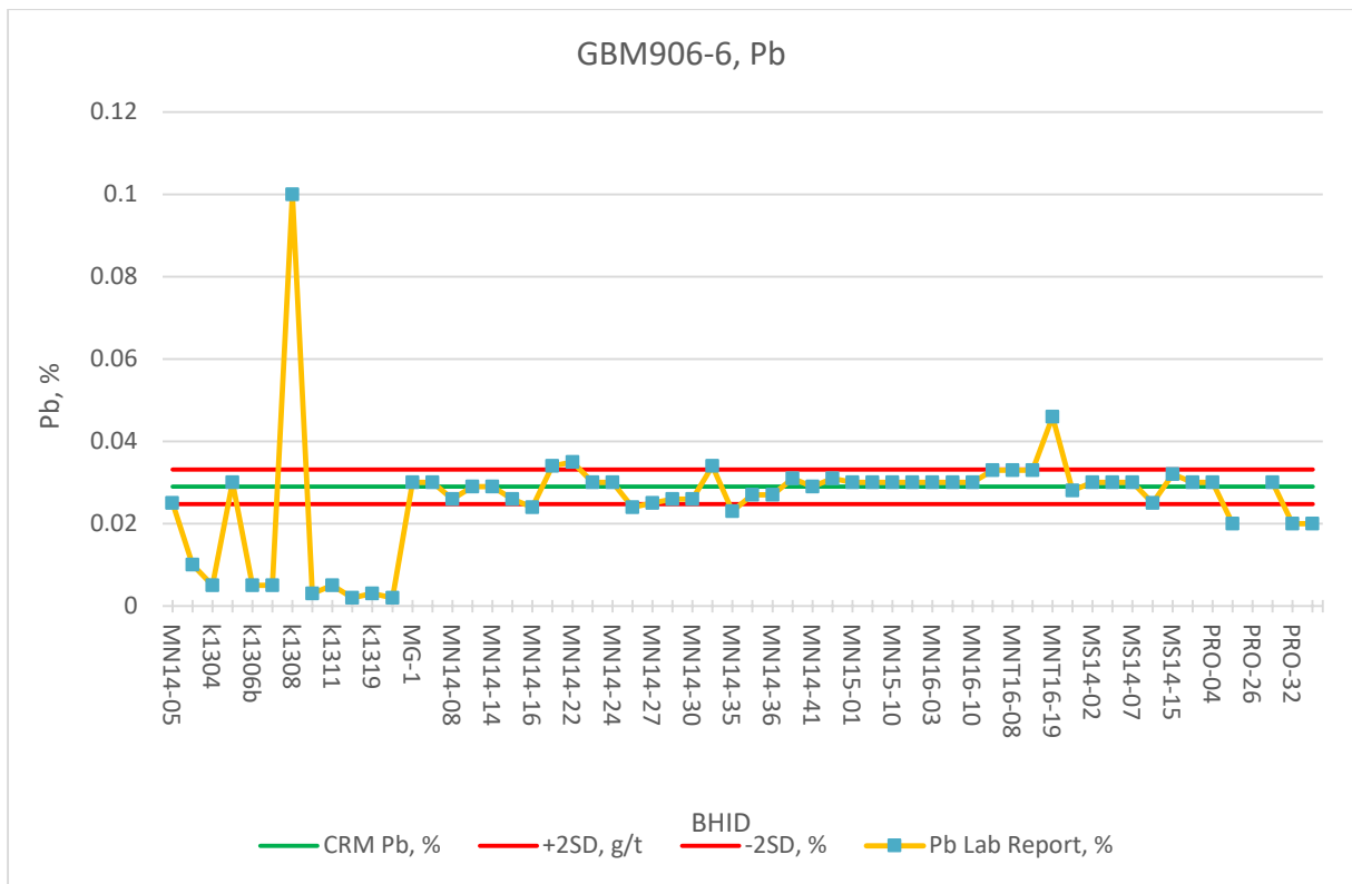
Figure 11.49: GBM 906-6, Pb, CRM Assaying Results
