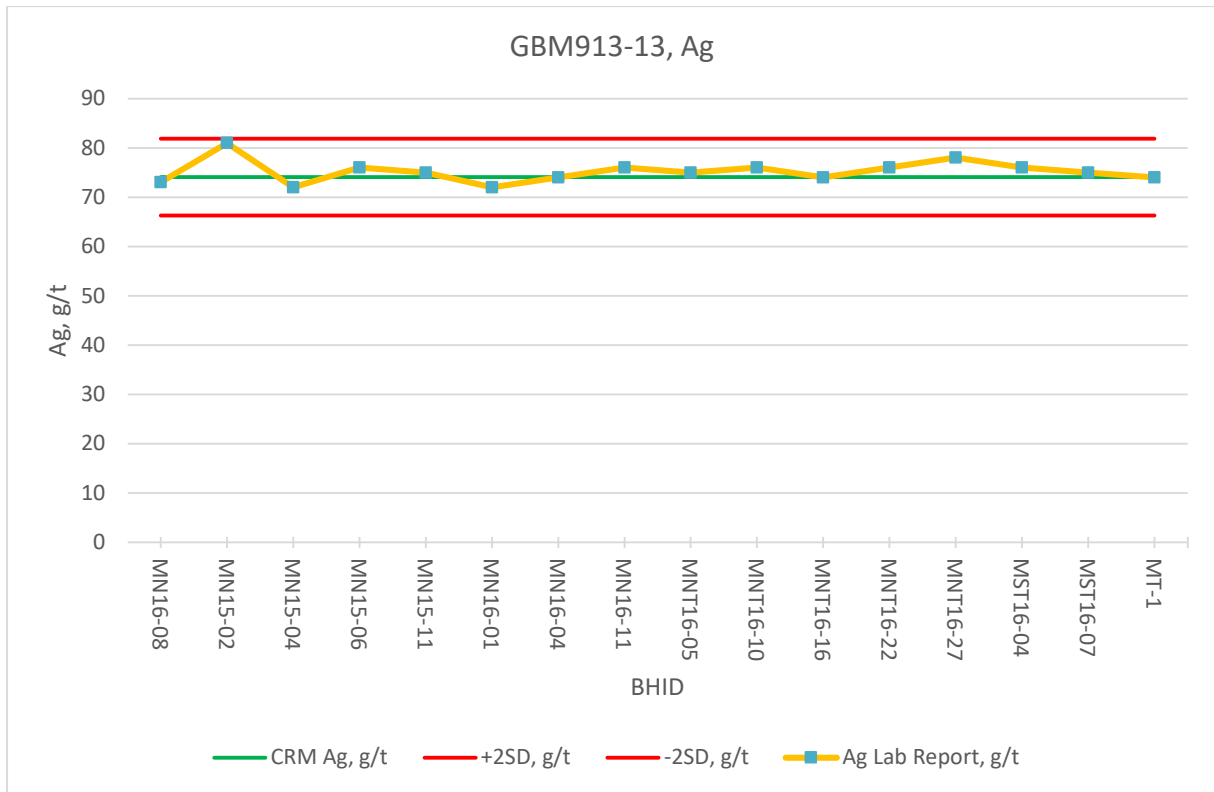
Figure 11.55: GBM 913-13, Ag, CRM Assaying Results
