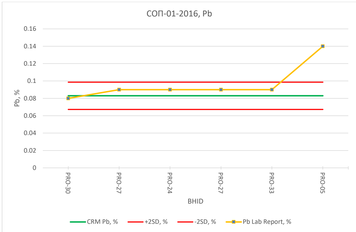
Figure 11.57: SOP-01-2016, Pb, CRM Assaying Results
