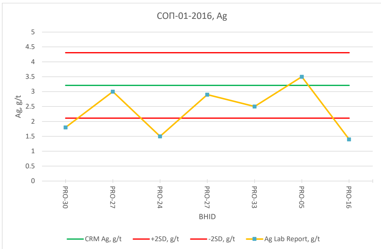
Figure 11.56: SOP-01-2016, Ag, CRM Assaying Results
