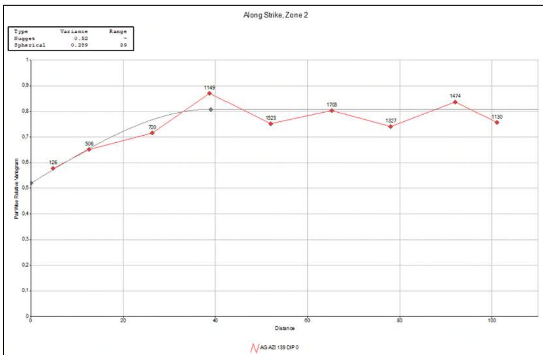
Figure 14.13: Ag Modelled Variogram, Zone 2, Along Strike
