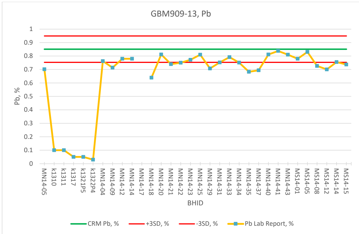
Figure 11.53: GBM 909-13, Pb, CRM Assaying Results
