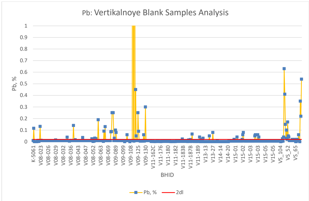
Figure 11.4: Blank Samples Analysed for Pb on Vertikalny
